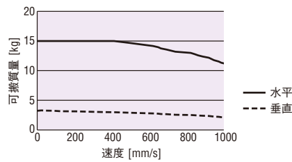
SKR4620A+AZM66MC (AC入力)
