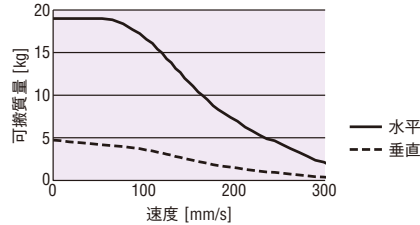
SKR2606A+AZM46MC (AC入力)
