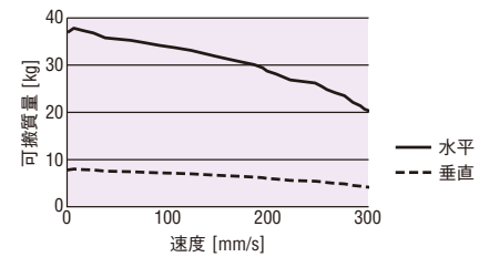
SKR3306A+AZM46MC (AC入力)
