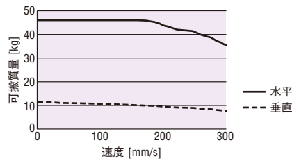
SKR2606A+AZM46MC (AC入力)
