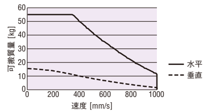
KR45H20A+AZM66MC (AC入力)
