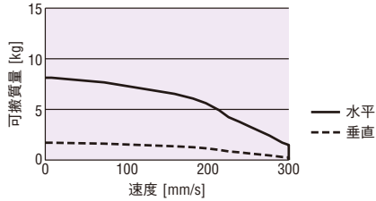
SKR2602A+AZM46MC (AC入力)
