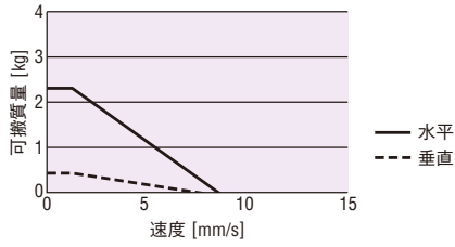
SKR2006A+AZM24AK (DC24V)
