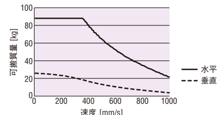
SKR4620A+AZM69MC (AC入力)
