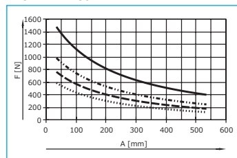
EAGF-V2-KF-80
