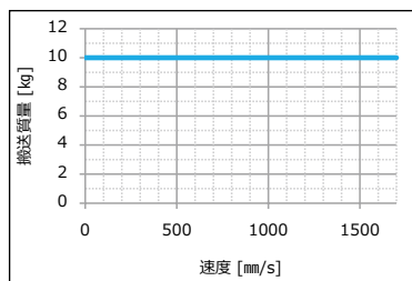
ELGR-TB-45
