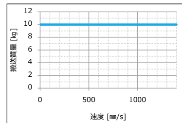
ELGG-TB-35※5
