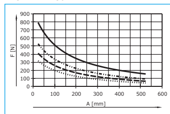
EAGF-V2-KF-50
