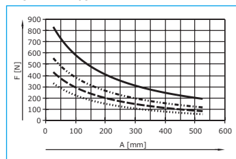
EAGF-V2-KF-63
